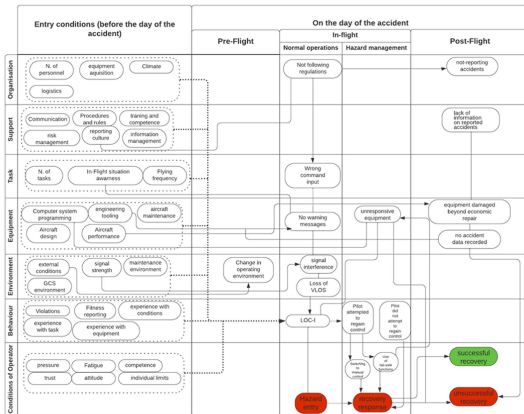
Figure 1: UAV LOC-I framework (adapted from ARM)
